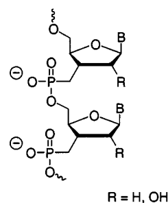
Figure 1. Internucleoside linkages with the 3'-oxygen replaced with a methylene group in the phosphodiester backbone
